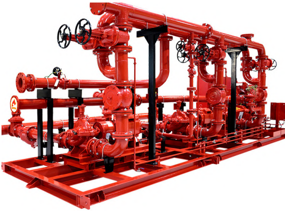
Fire pumps
